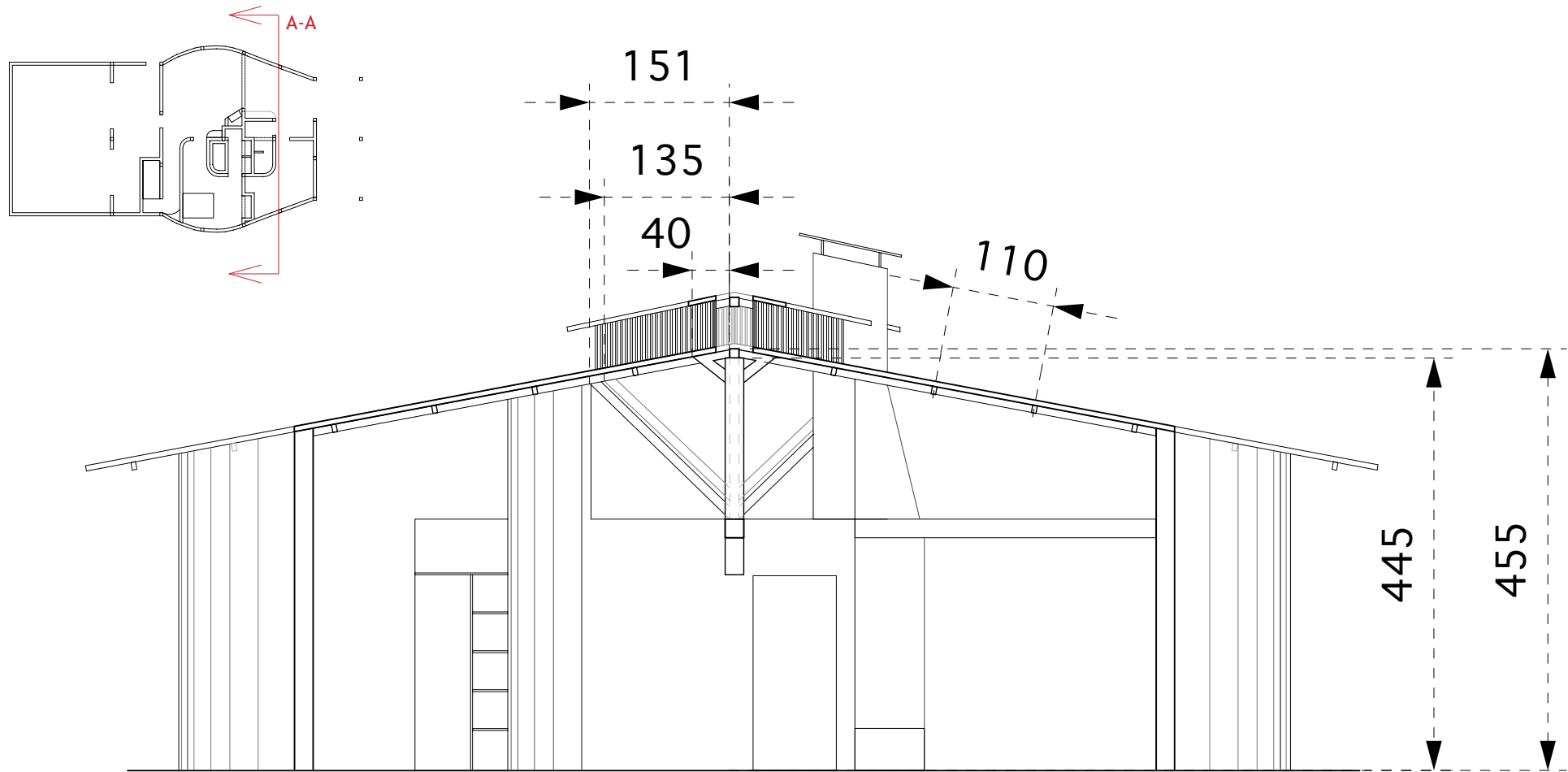
cross section A-A skylight + main roof beam structure and spacing
